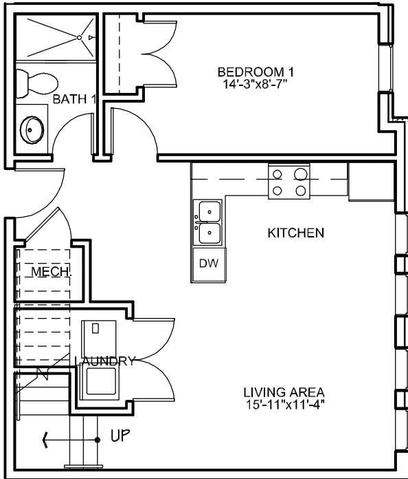
LOWER LEVEL
