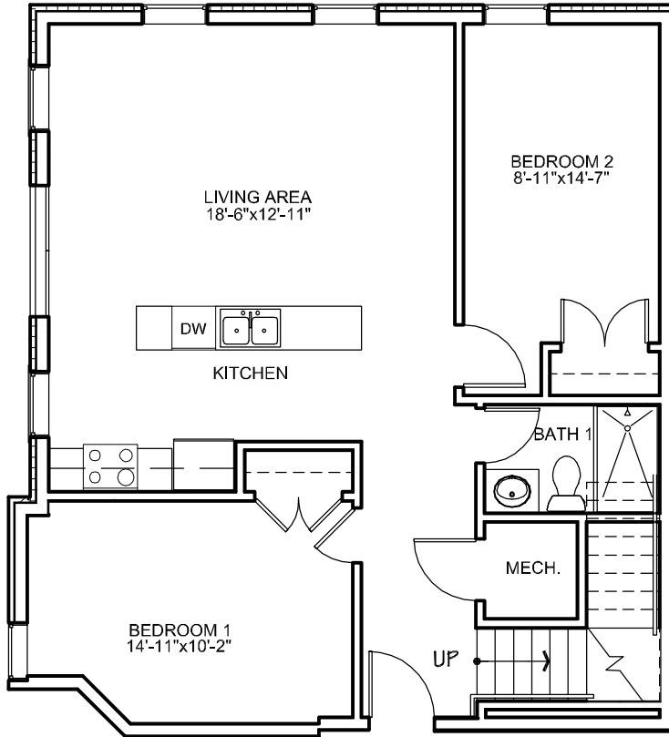
LOWER LEVEL
